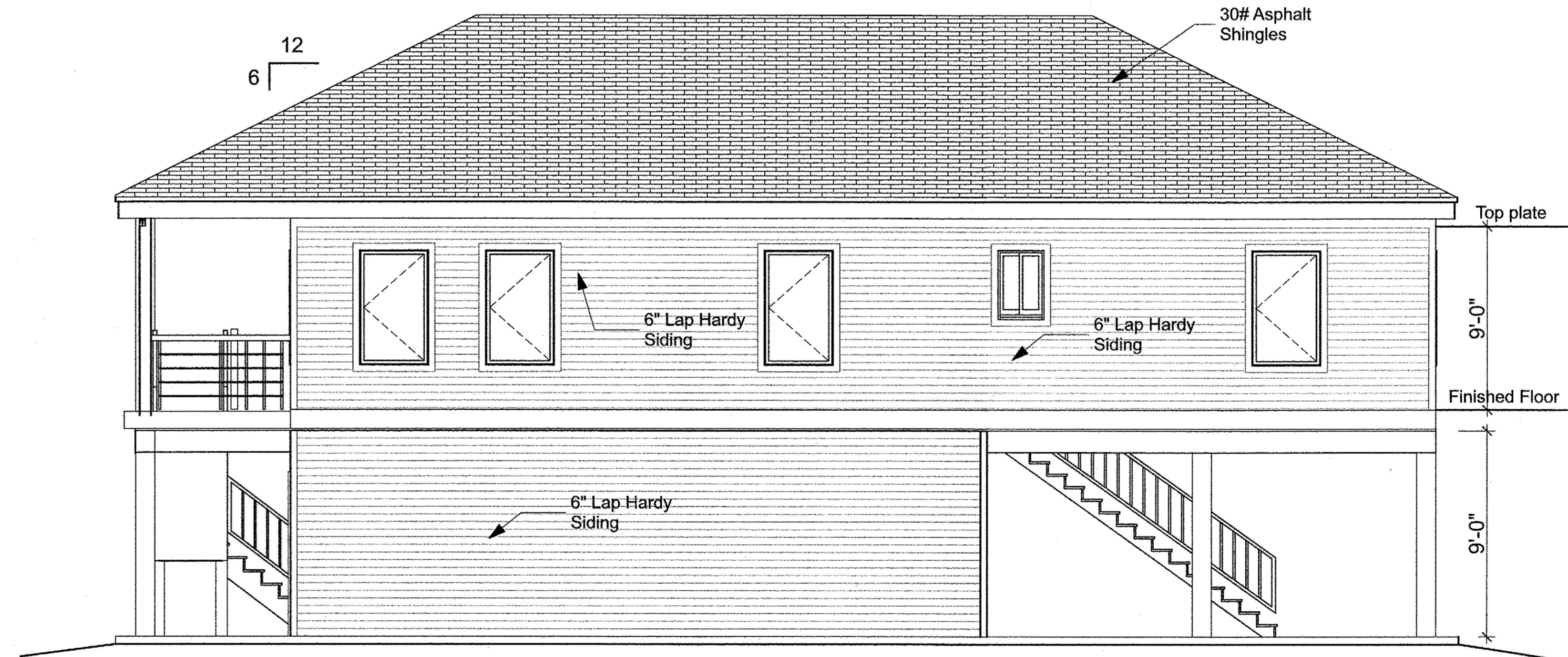
SOUTH ELEVATION
