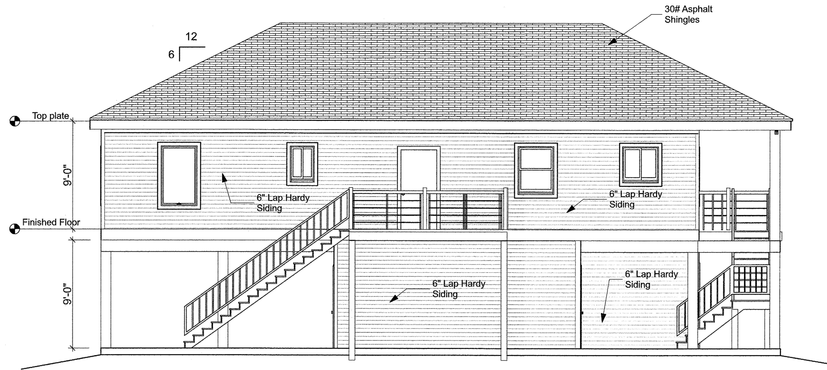
NORTH ELEVATION
