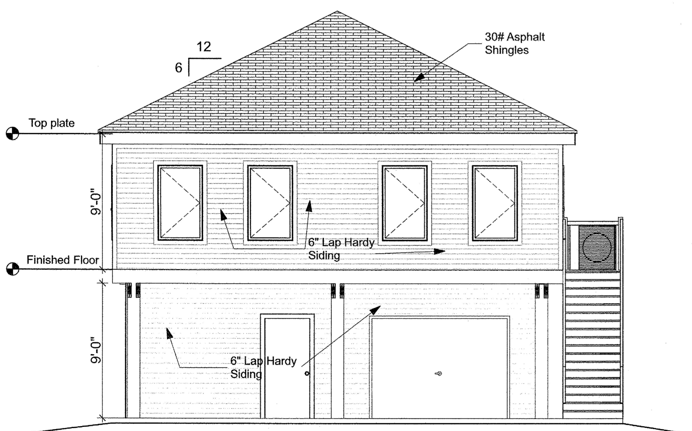
EAST ELEVATION
