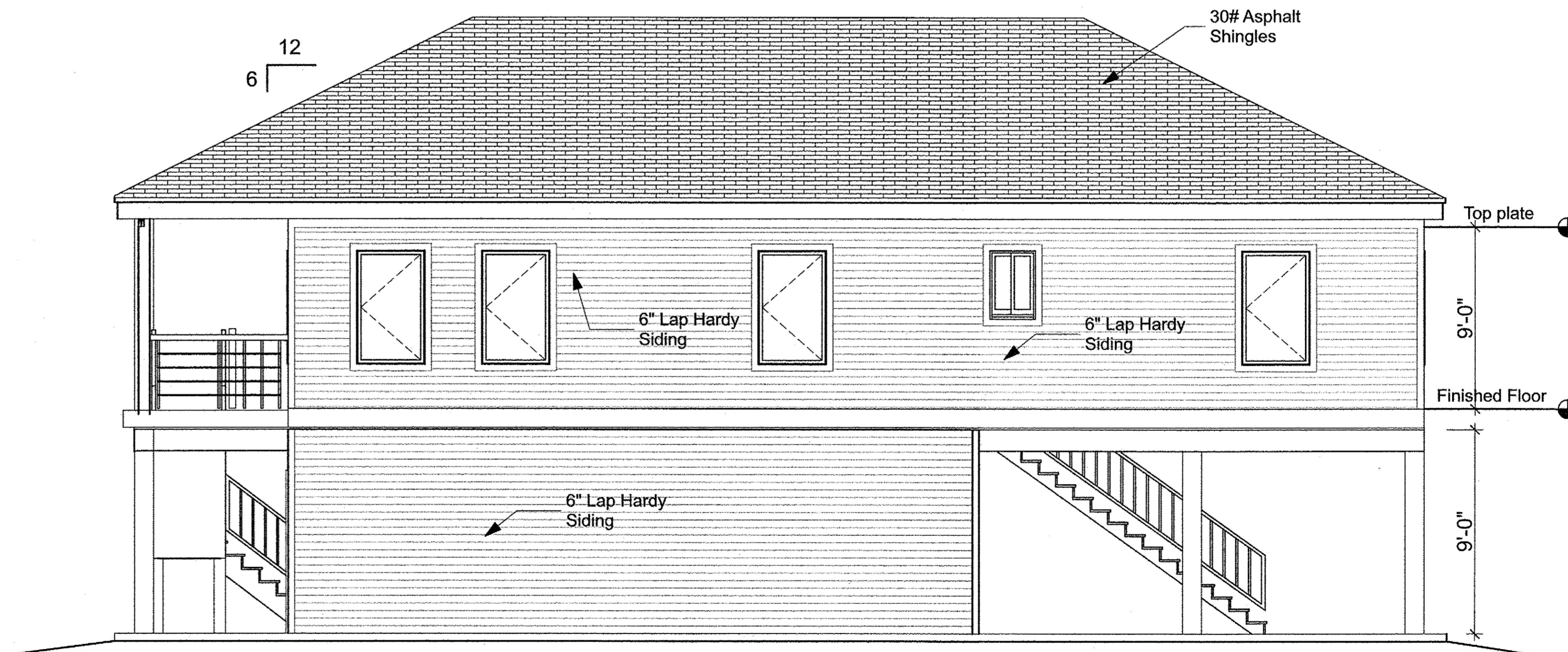
SOUTH ELEVATION
