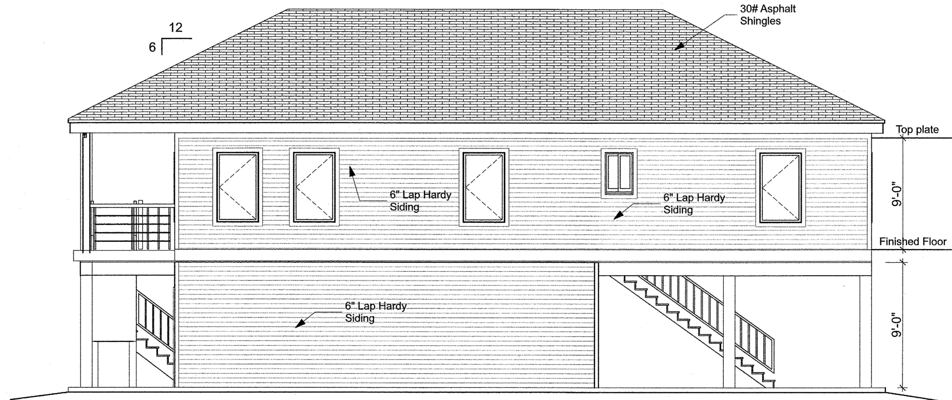
SOUTH ELEVATION
